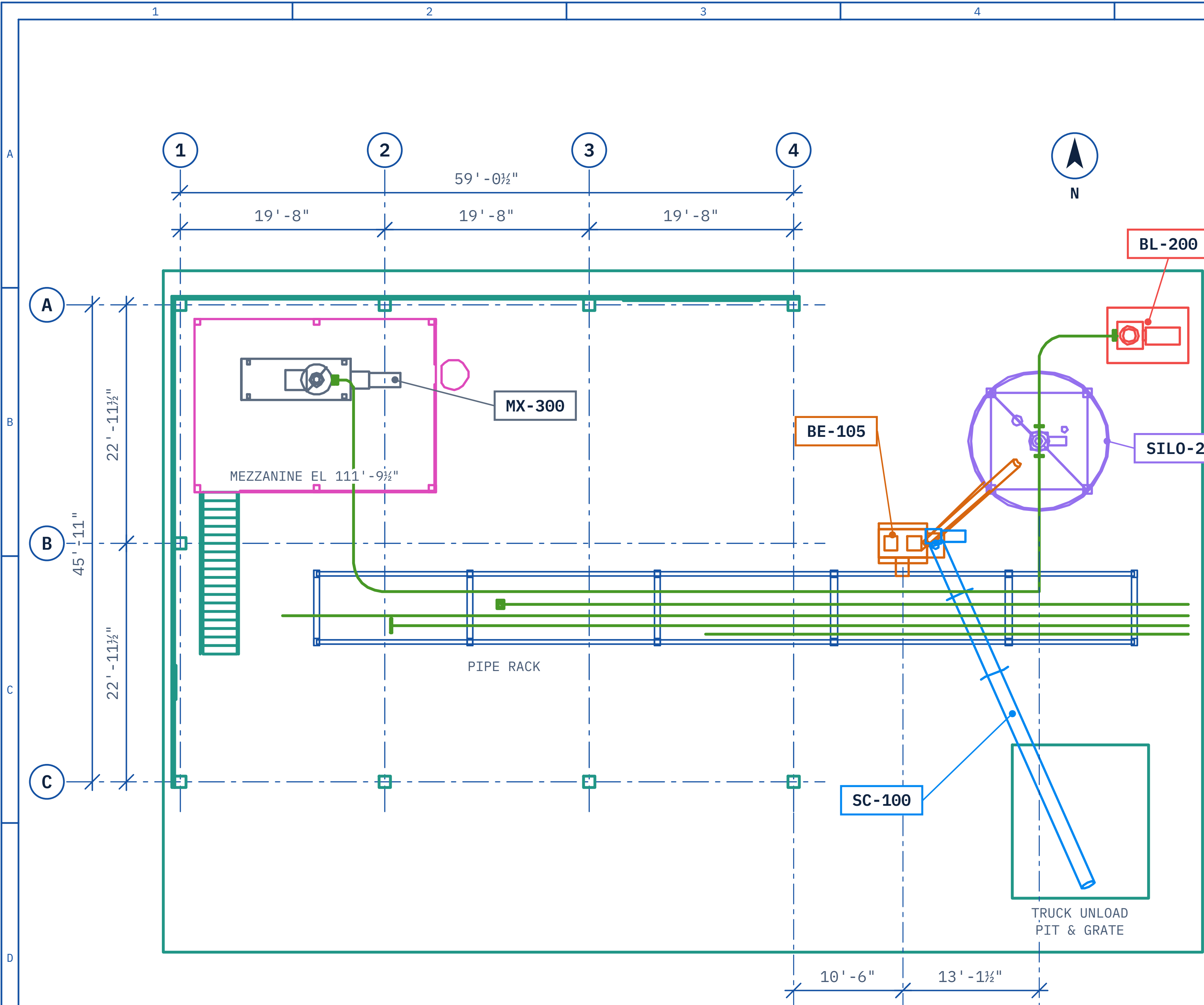
1 PLAN – EQUIPMENT LAYOUT SCALE: NTS
