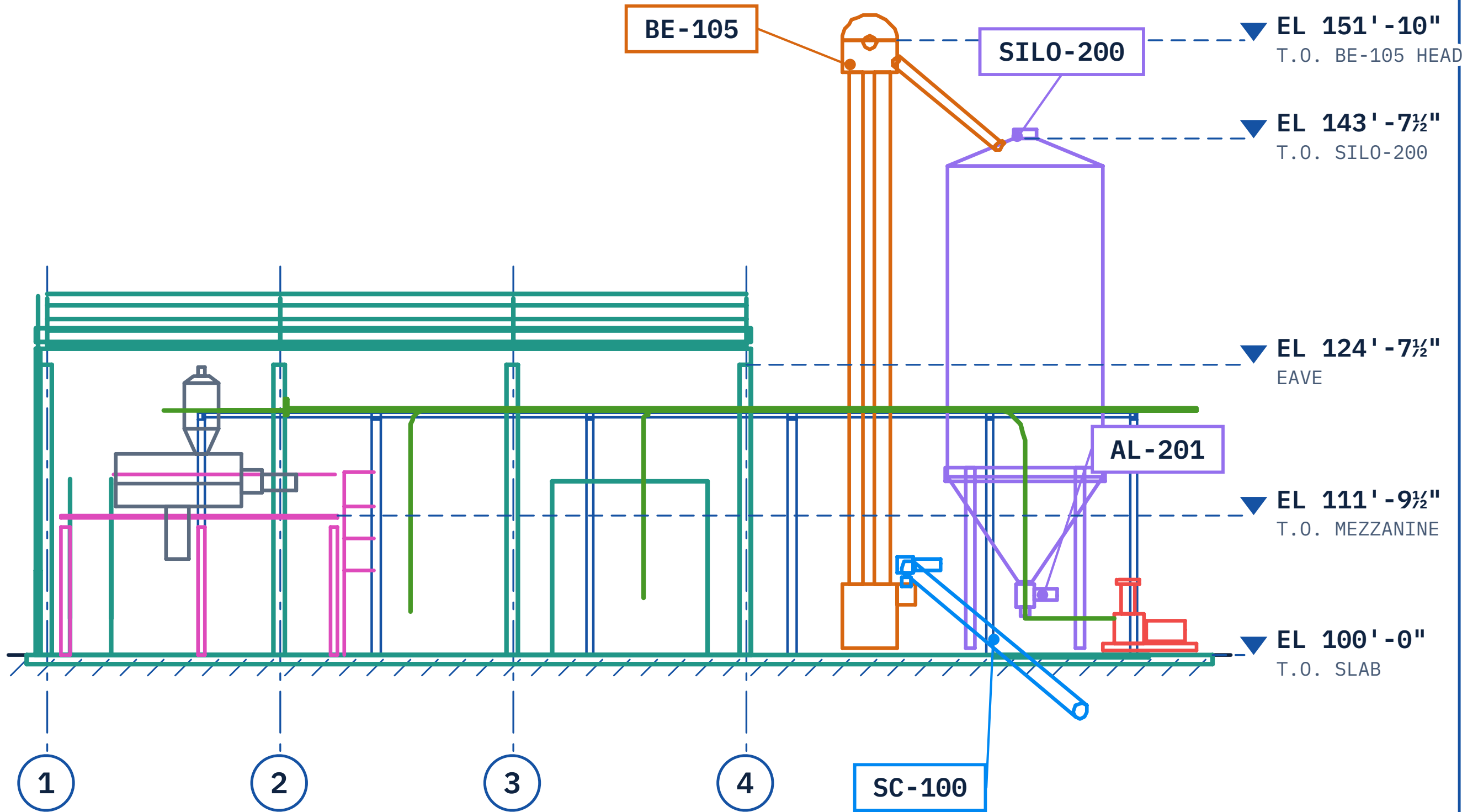
2 ELEVATION A – LOOKING NORTH SCALE: NTS
